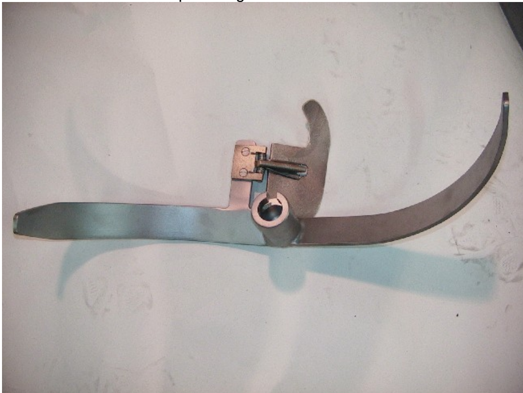
EXHIBIT E - Special Agitator/Mixer for Caramel Corn
