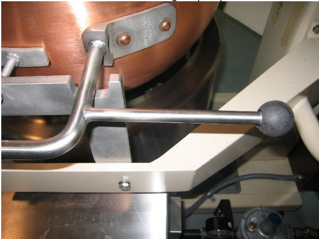
EXHIBIT C - In-Place kettle tilting for quick product removal
